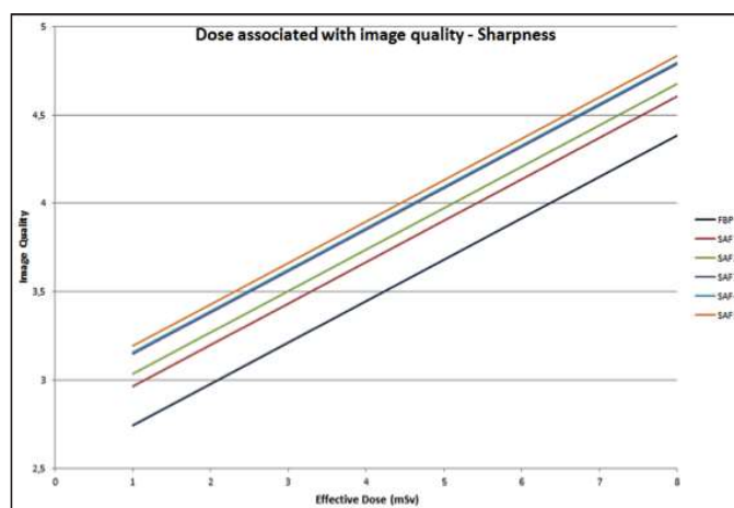
Figure 1: linear regression for sharpness for SAFIRE and FBP.
